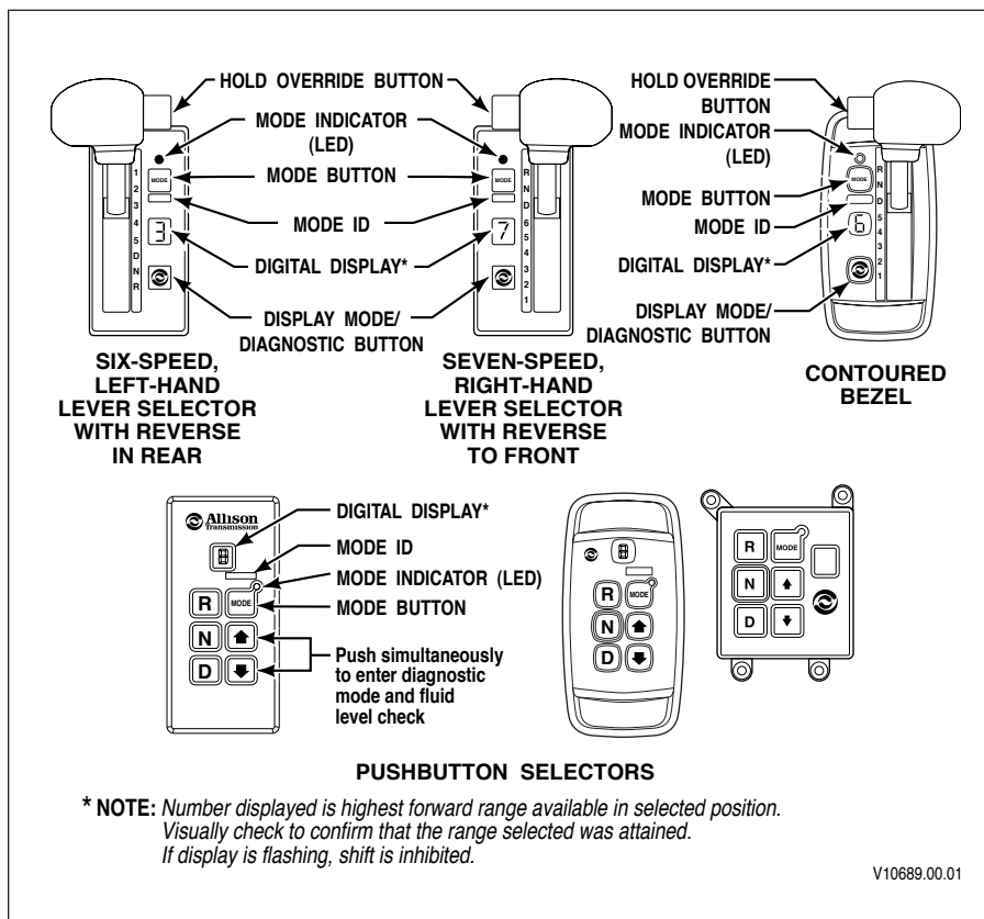
Figure 6. Typical WTEC III Allison Shift Selectors
